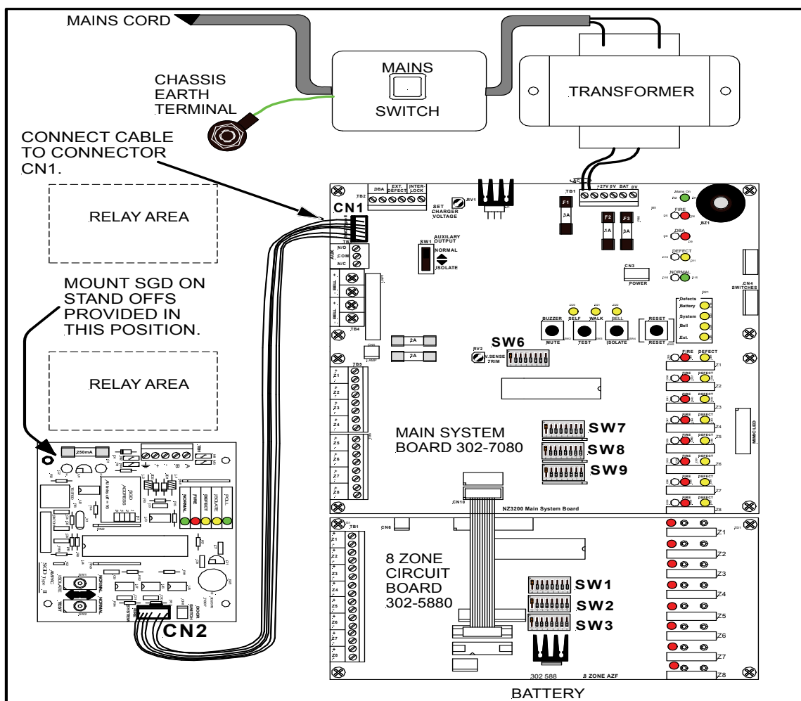
Figure 1: SGDII Typical Wiring Layout
