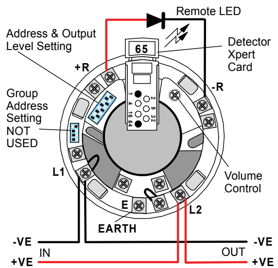
Figure 2: Integrated Base Loop Sounder Wiring
