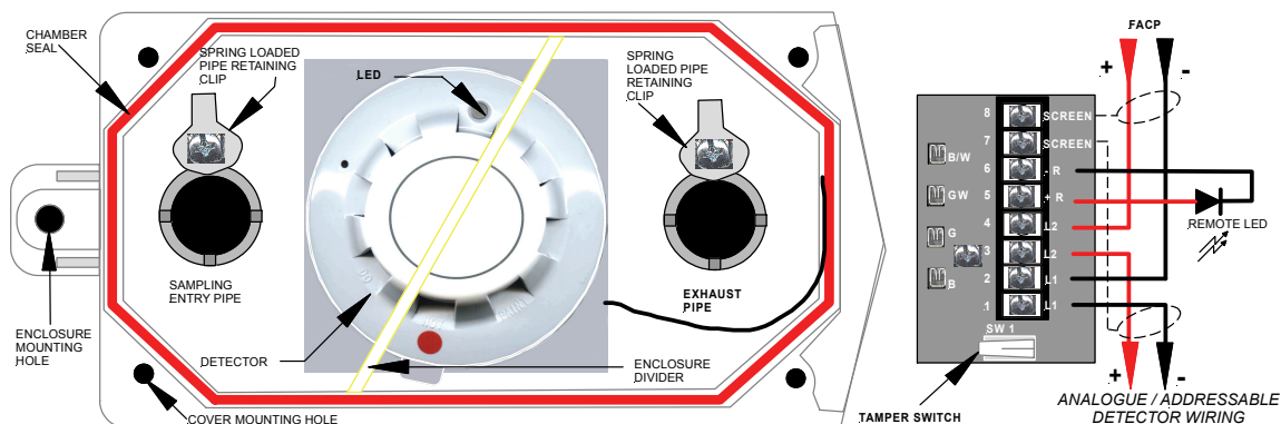
Figure 3: Cutaway View of the Enclosure, Terminal Block & Wiring Diagram
