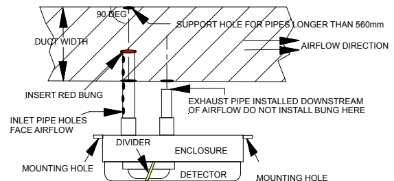
Figure 2: Detector Duct Installation
