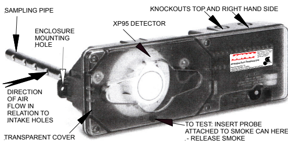
Figure 1: Duct Sampling Unit
