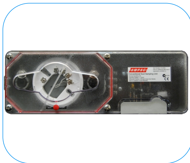
Duct Sampling Unit cw Orbis Detector Base
