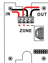
Figure 3: 4255-0700 c/w Conventional Interface
