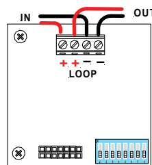
Figure 2: 4255-0600 c/w Addressable Interface
