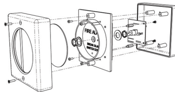
Figure 2: 4255-0600 c/w Addressable Interface
