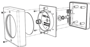
Figure 1: 4255-0500, 4255-0510 c/w Toggle Switch
