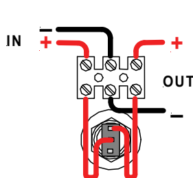
Figure 1: 4255-0500, 4255-0510 c/w Toggle Switch
