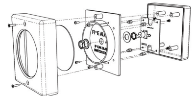
Figure 3: 4255-0700 c/w Conventional Interface
