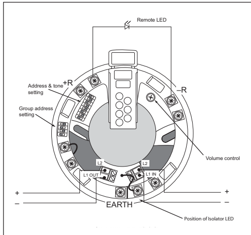
Fig. 2 XP95 Integrated Base Sounder with isolator wiring
