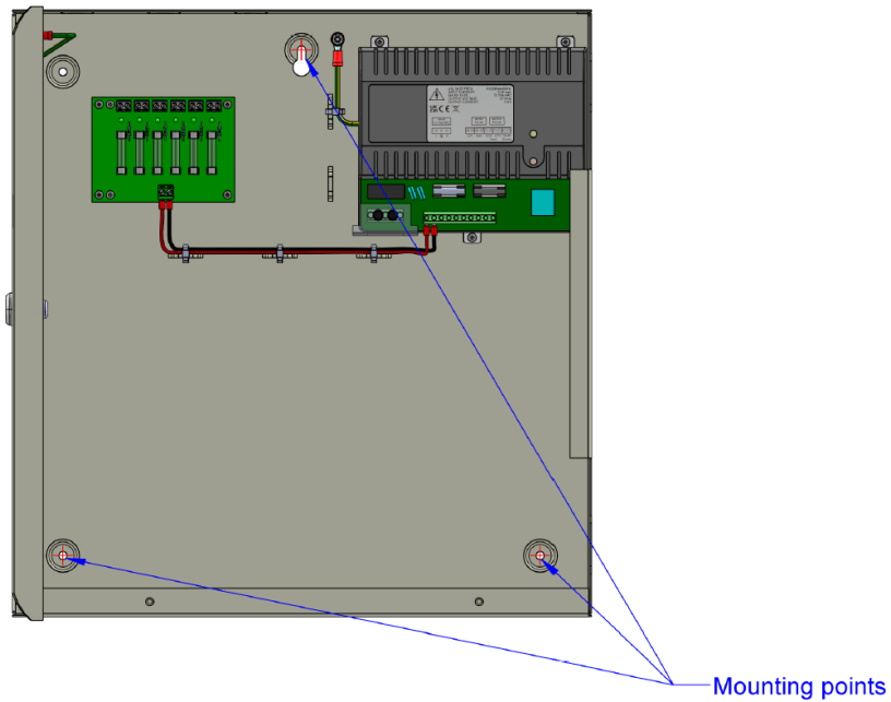
Figure 1 - Box mounting
