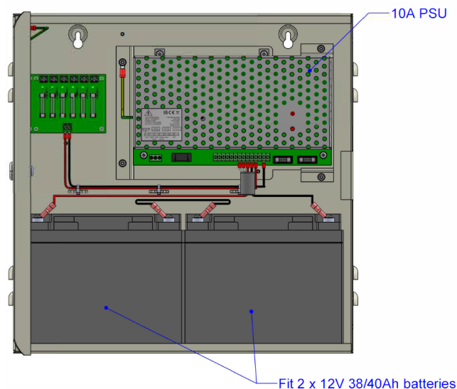
Figure 2 - Battery fitting and assembly
