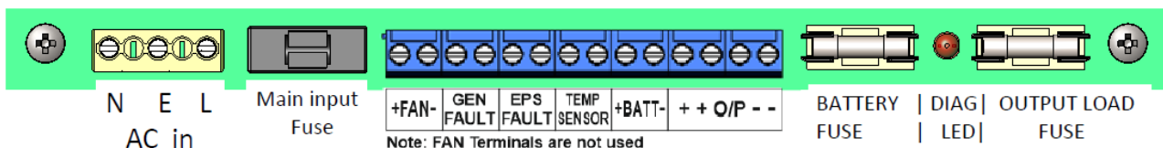
Figure 6 - Terminal labels
