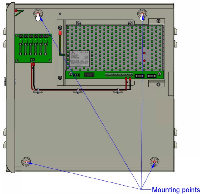
Figure 1 - Box mounting
