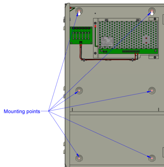
Figure 3 - Box and Battery box mounting
