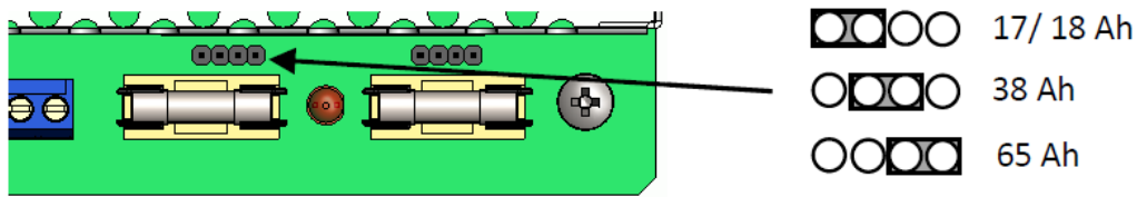
Figure 7 - Standby battery size selection links
